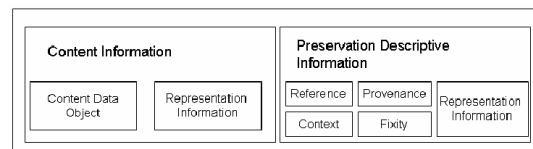
Figure 1 - AIP structure in OAIS [1]
